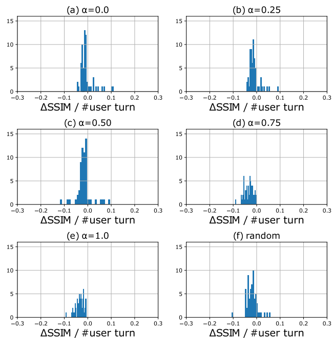
FIGURE 3. Histogram of \Delta SSIM / \#user\ turn at end of dialogues on each strategy: higher \Delta SSIM / \#user\ turn dialogue created more similar images to goal and more efficient dialogues.
