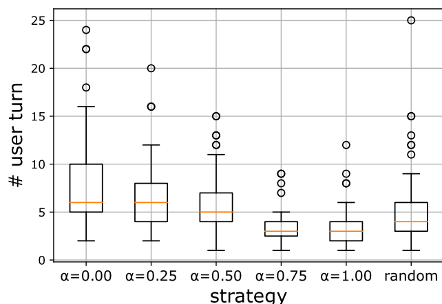
FIGURE 4. Distribution of \#user\ turn on each strategy: smaller \#user\ turn dialogue represents more efficient dialogue.
