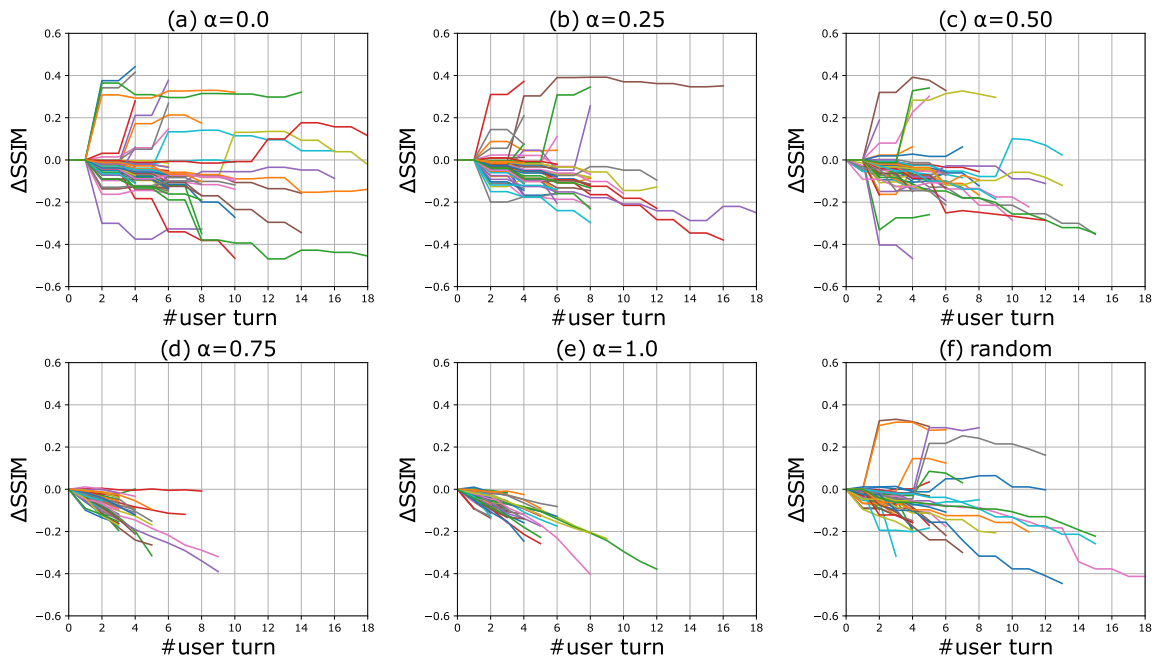
FIGURE 2. Experimental results of image editing dialogue between 18 evaluators (users) and the system: #user turn denotes total number of user actions ( making an editing request and selecting an image ); (smaller is better). \Delta SSIM denotes current source-goal SSIM, subtracted by first source-goal SSIM (higher is better). Each plot in figures represents each dialogue sample. \alpha indicates threshold for system to select confirmation: (a) \alpha = 0.0 , (b) \alpha = 0.25 , (c) \alpha = 0.50 , (d) \alpha = 0.75 , (e) \alpha = 1.0 , and (f) random: system randomly selects confirmation. If \alpha becomes smaller, system tends to select confirmation with a lower uncertainty score. Note that every \Delta SSIM is calculated after the user's action. Therefore, when the system selects confirmation after the user makes an editing request, \Delta SSIM keeps the same value. Degradation as dialogues progress is caused by image editing models.
